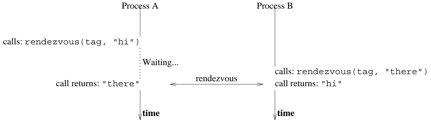
Figure 10.8: Two processes doing a rendezvous.
